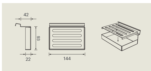
SOAP DISH
